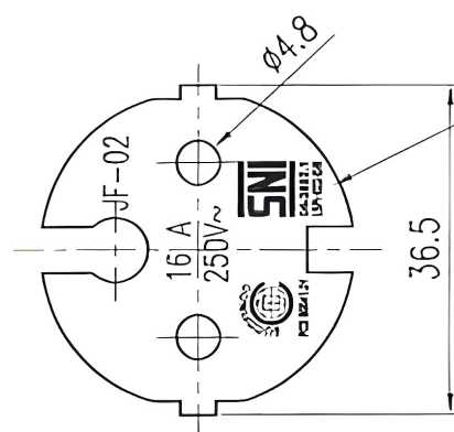
VIEW-B
